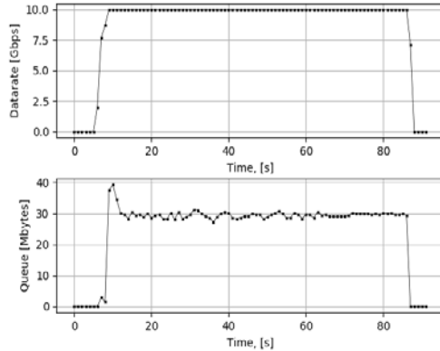
Figure 5: Test 3: BBW 10 Gbps, base RTT 100 ms, single flow.
