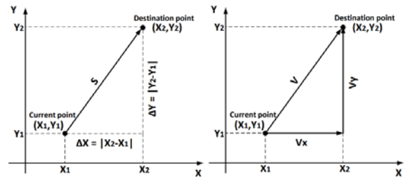
Figure 8: Interpolation of distance and velocity between two points.
