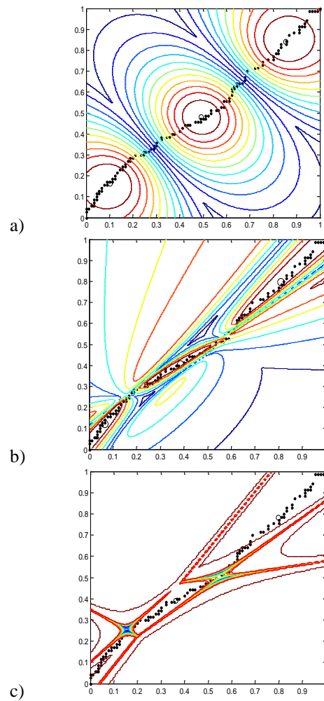
Figure 3: Fuzzy clustering of data on the POTE elements temperature, FCM (PC=0.82, CE=0.34) (a), GK (PC=0.91, CE=0.18) (b), GG (PC=0.96, CE=0.07) (c).
