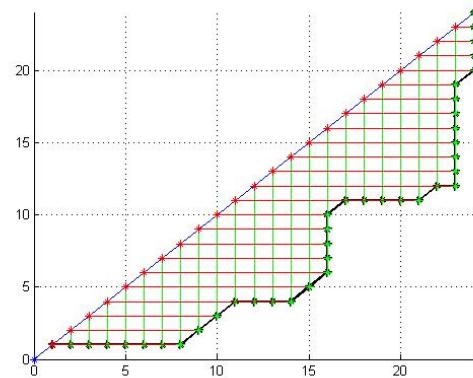
Figure 5: Warping patch along with diagonal for classical DTW. Lines show distances between path and diagonal.
