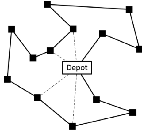
Figure 2: The total cost of the solution is reduced by connecting routes into one.
