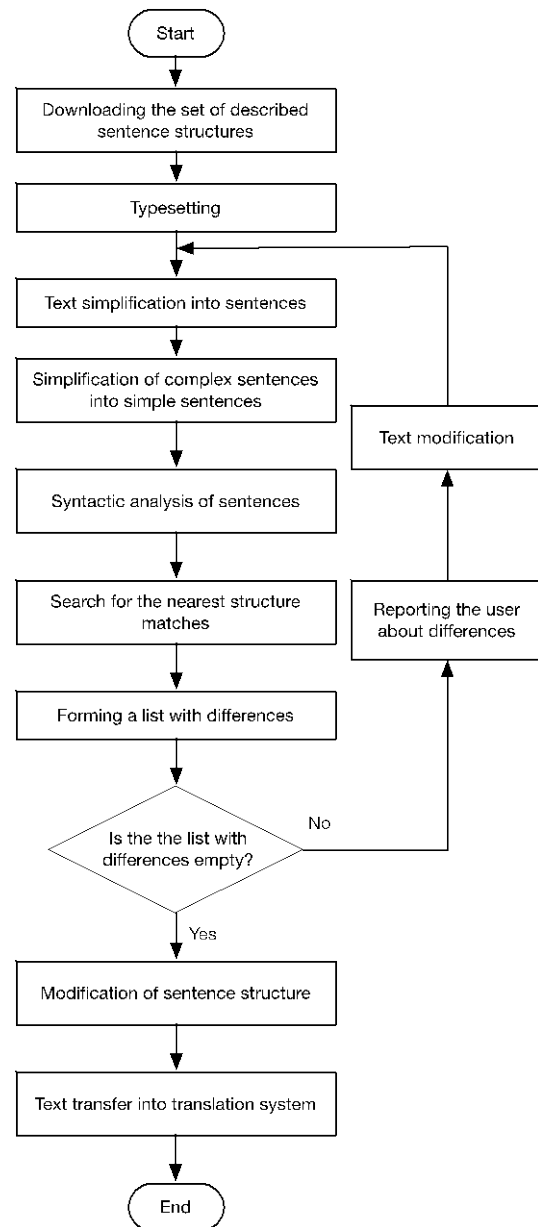
Figure 2: The algorithm of using the description language for language structures.
