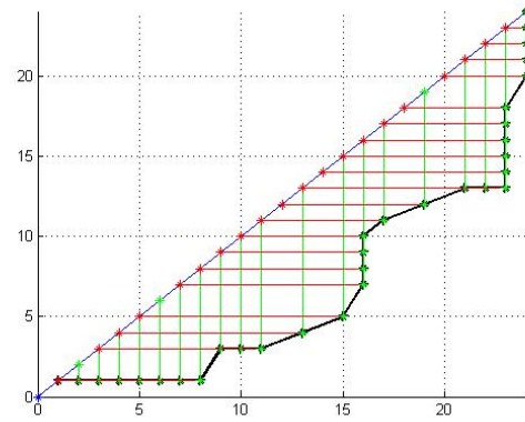
Figure 8: Warping patch along with diagonal for modified DTW. Lines show distances between path and diagonal.
