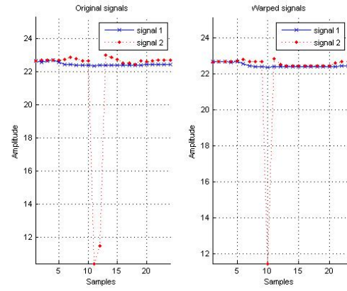
Figure 12: Warping diagrams for modified DTW. Left graph – signals before warping, right graph – signals after warping.
