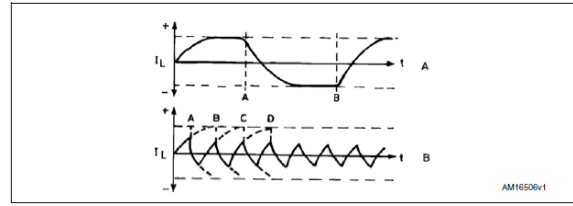
Figure 3: Peak winding current decreasing at higher speed, limited by motor inductance [9].
