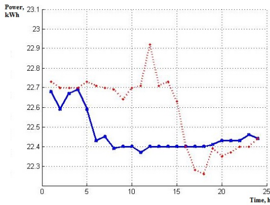
Figure 2: Power consumption profile of oil well. Dotted line - reference signal, solid line - test one.
