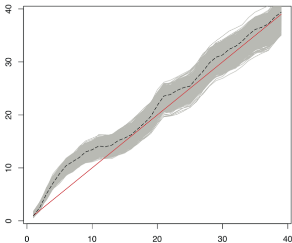
Figure 5: The reduced criterion variation obtained using the fractal forecast method.
