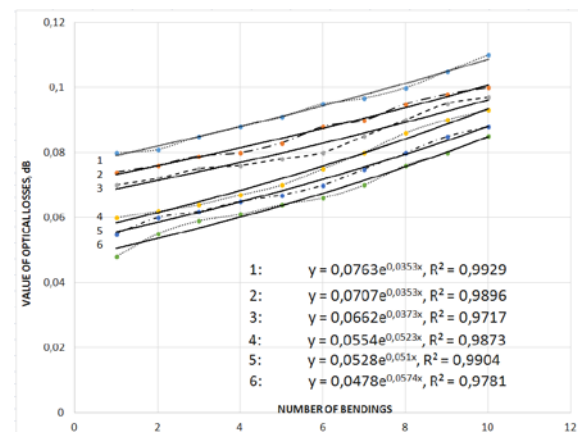
Figure 2: The value of the optical loss of SNR-UT-12 fiber optic cable. The value of the radius r for the curves: 1: 3 mm, 2: 5 mm, 3: 10 mm, 4: 12 mm, 5: 15 mm, 6: 18 mm.
