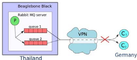
Figure 5: Disconnect of consumers.
