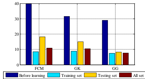
Figure 6: Results of the evaluation of the accuracy of fuzzy models of diagnostics of the POTE. The average number of misidentified MCE states, %.
