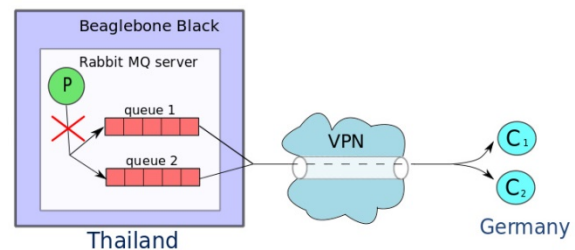
Figure 6: Crash of Rabbit MQ producer and server.
