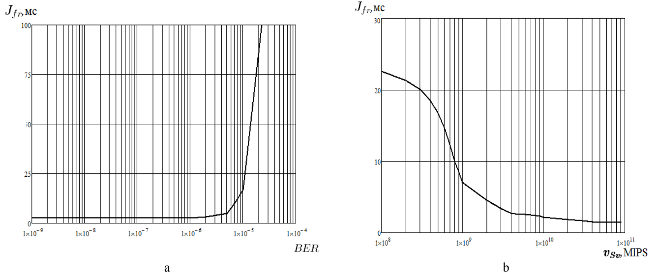
Figure 4. Dependence of jitter: a) - the intensity of the bit error rate, b) - the performance of the server
