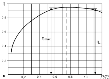
Figure 2: Dependence of the efficiency of the ATM on the load.
